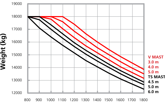
180D-9B Load Center (mm)
