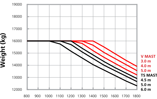
160D-9L Load Center (mm)
