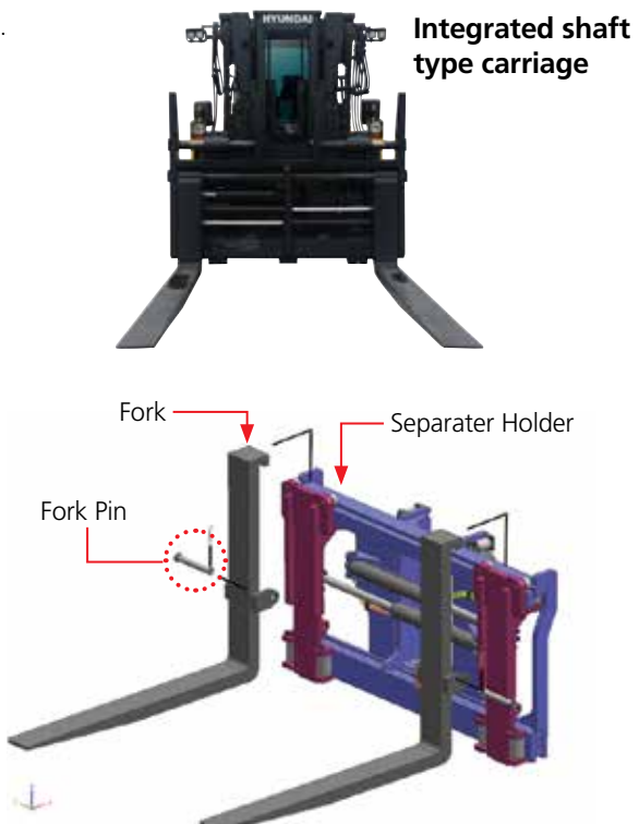
Separator Holder Type Fork Carriage (Optional) To improve handling and easily switch forks and other attachment Separator holder system is adopted as option. It is possible to install various attachments like coil ram easily.
